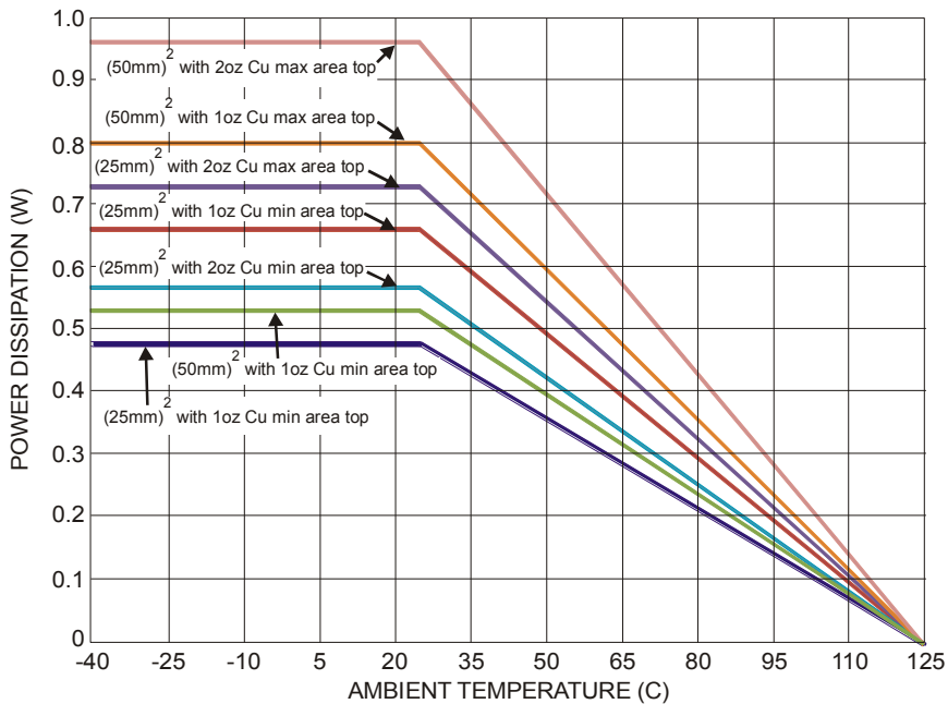
Figure 42. Derating Curve for Different PCB
